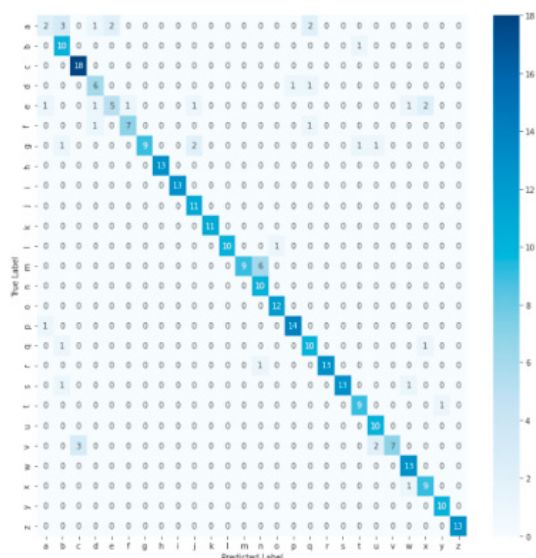
Fig. 10. Confusion matrix for sign language dataset using LSTM
