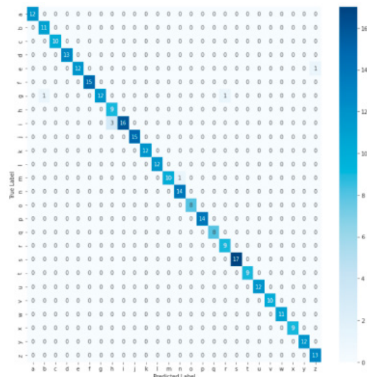
Fig. 9. Confusion matrix for sign language dataset using CNN
