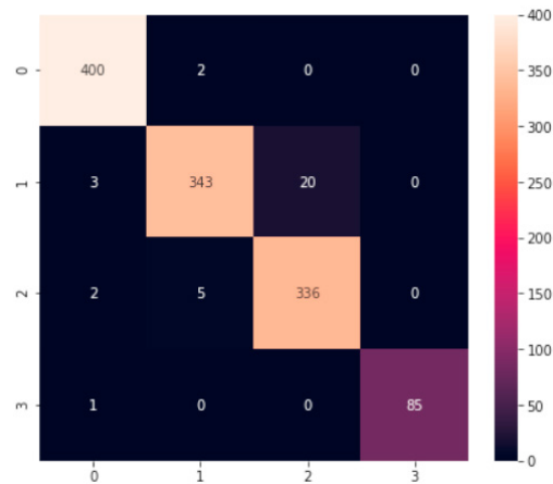
Fig. 6. Confusion matrix with 1200 samples
