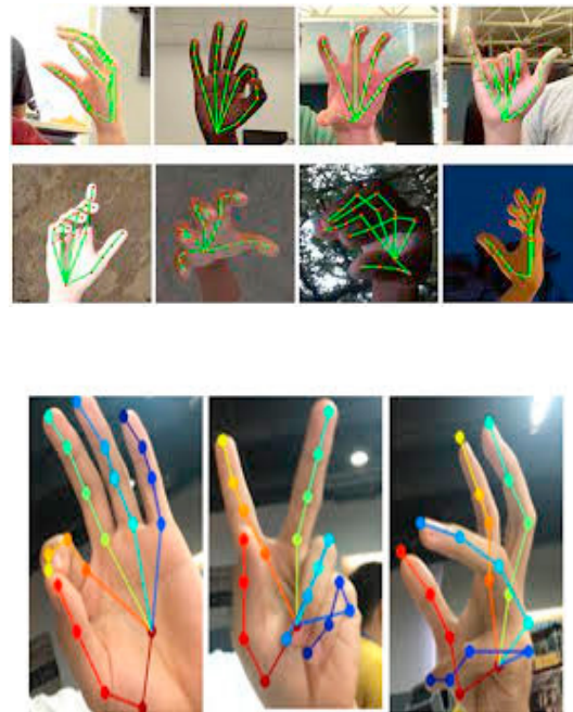
Fig. 5. Keypoint detection
